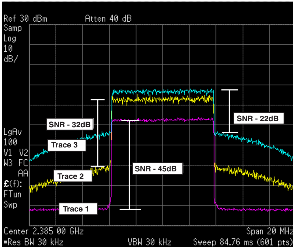
Fig. 1: OFDM signal spectrum showing increasing IMD as amplifier enters gain compression
